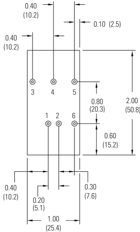
BOTTOM VIEW
